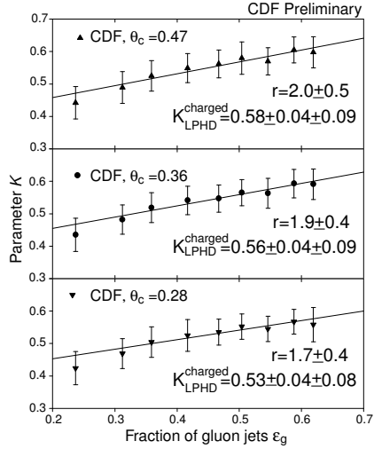
Figure 3. Parameter K extracted from the fits of momentum distributions for each dijet mass bin as a function of the fraction of gluon jets in the bin. Parton-to-hadron conversion ratio K_{LPHD} and the ratio of multiplicities in gluon and quark jets is extracted from a linear fit. Three plots correspond to three cone-sizes \theta_c .
