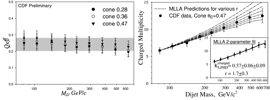
Figure 2. Left: Result of the fits of the momentum distributions for the MLLA cut-off parameter Q_{eff} . The data points correspond to the available combinations of the dijet mass and cone-sizes. Right: Measured multiplicity of charged particles in jets for cone-size \theta_c=0.47 . The result is fitted for LPHD parameter K_{LPHD} and the ratio of charged particle multiplicities in gluon and quark jets (insert).
