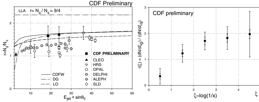
Figure 4. Left: Model-independent ratio r of multiplicities of charged particles in gluon and quark jets as a function of jet hardness. Also shown are earlier experimental results and theoretical predictions. Right: The ratio of momentum distributions of charged particles in gluon and quark jets for the bin with mean jet energy of 40 GeV.
