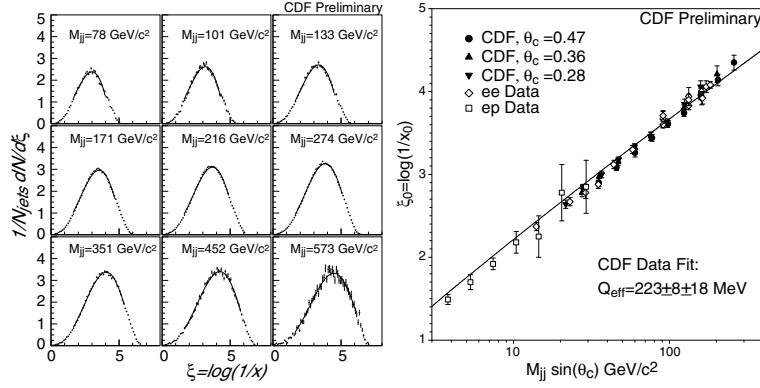
Figure 1. Left: Momentum distribution of charged particles in jets within cone of \theta_c = 0.47 rad around the dijet axis. Data was fitted with the MLLA spectrum for Q_{eff} and K . Right: Peak position of the momentum distribution vs M_{jj} \sin \theta_c verifies the scaling predicted by MLLA.
