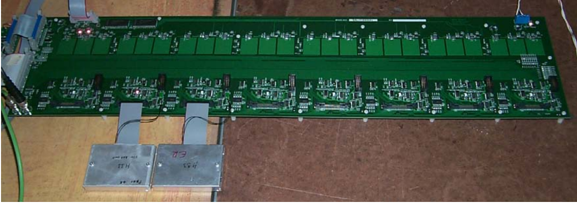
Figure 7: The MPX board distributes initialization and control signals, including the burn-in pattern, to the eight hybrid ports that can be seen along the lower edge of this photograph (only two hybrids are connected at this time). It also distributes analog and digital voltage to the hybrids, selects among hybrids for data readout, and selects among hybrids for current and voltage monitoring.
